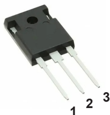
TO-247 MUR6040PT
