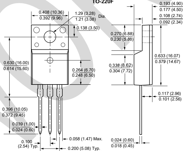
TO-220F
