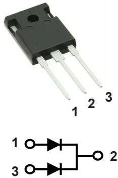
TO-247 MUR4040PT
