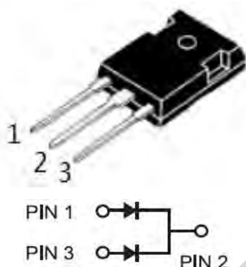
TO-247 TSR40L45PT
